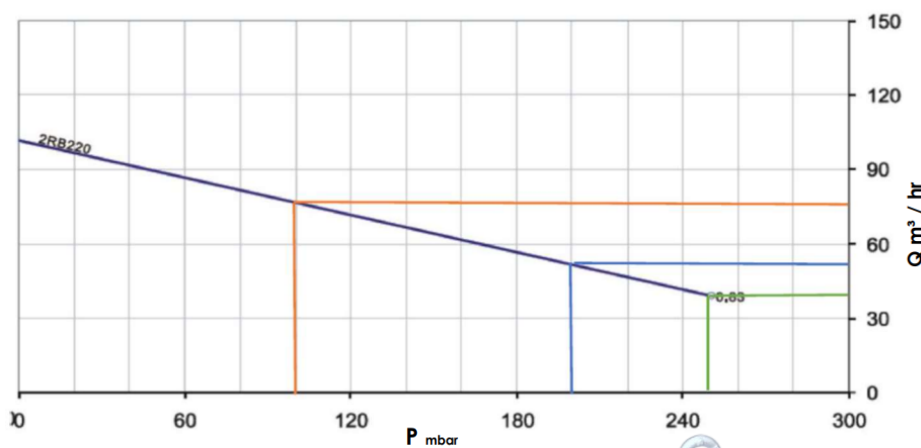
Compressor Selection Diagram 60Hz
